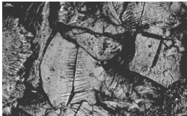
Figure 4 – Brittle and plastic deformation in a single coal particle
